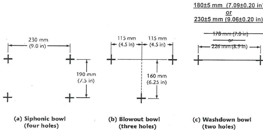
Figure 4 Bolt hole spacing for wall-mounted water closet bowls (See Clause 4.6.3.)
