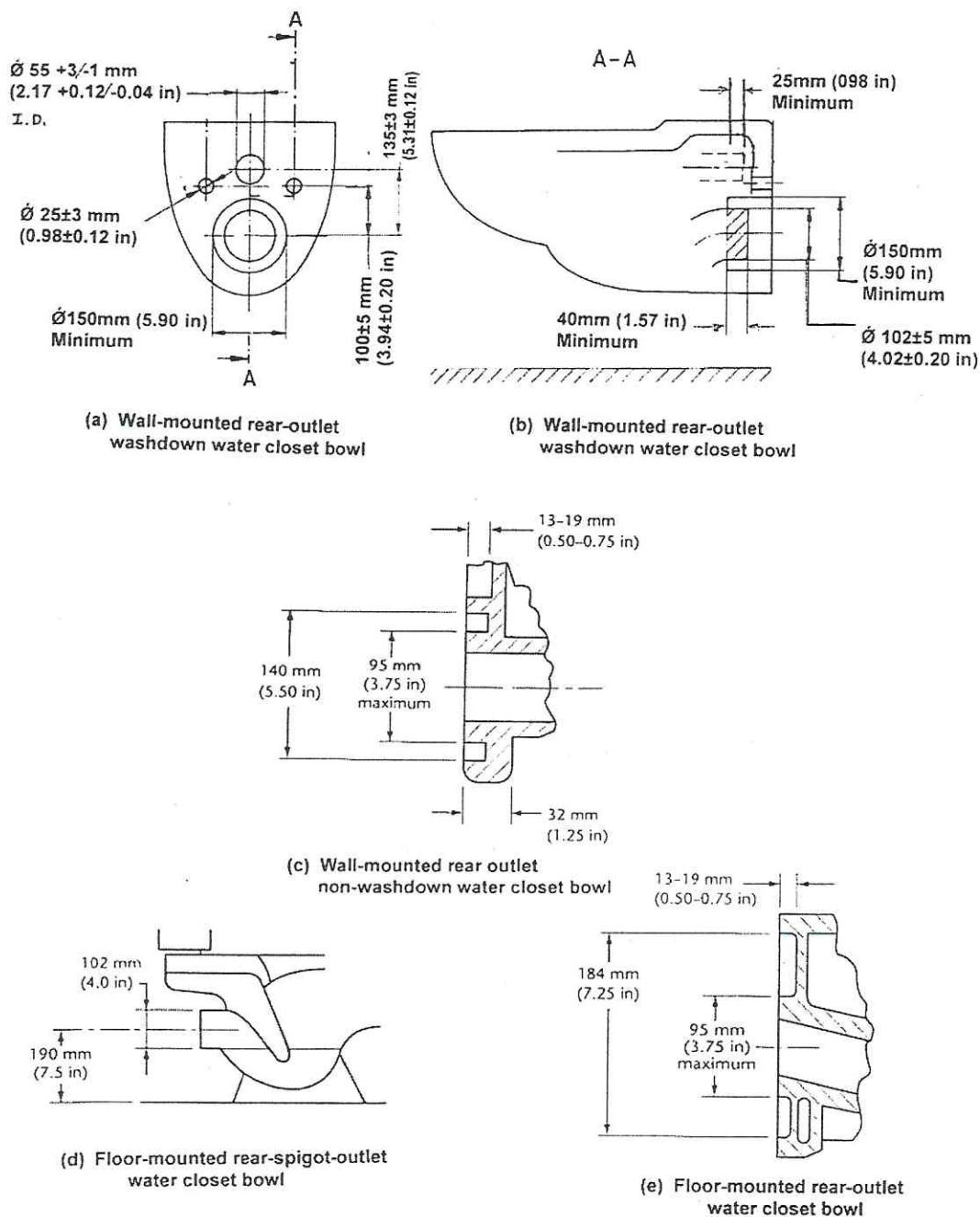
Figure 3 Outlet dimensions for rear-outlet and rear-spigot-outlet water closet bowls (See Clause 4.6.1.)
