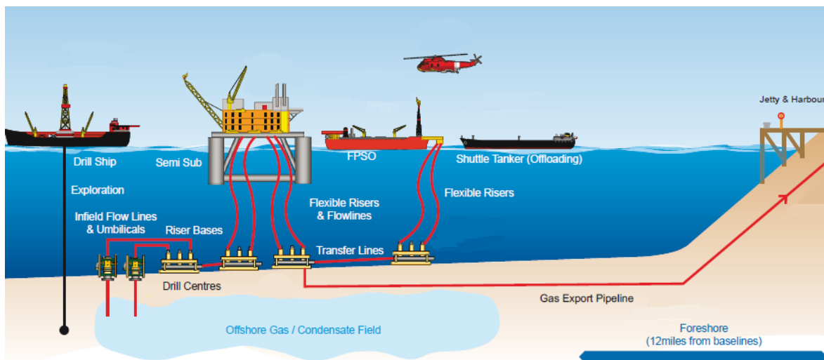
Figure 2.20: Example of subsea network for offshore oil and gas installations
