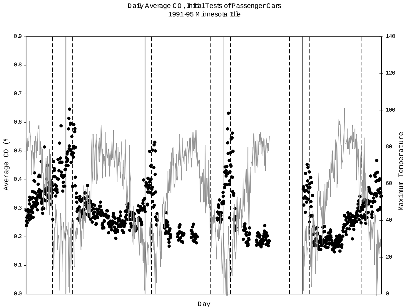
Figure 5.8. Daily Average CO, Minnesota Idle
