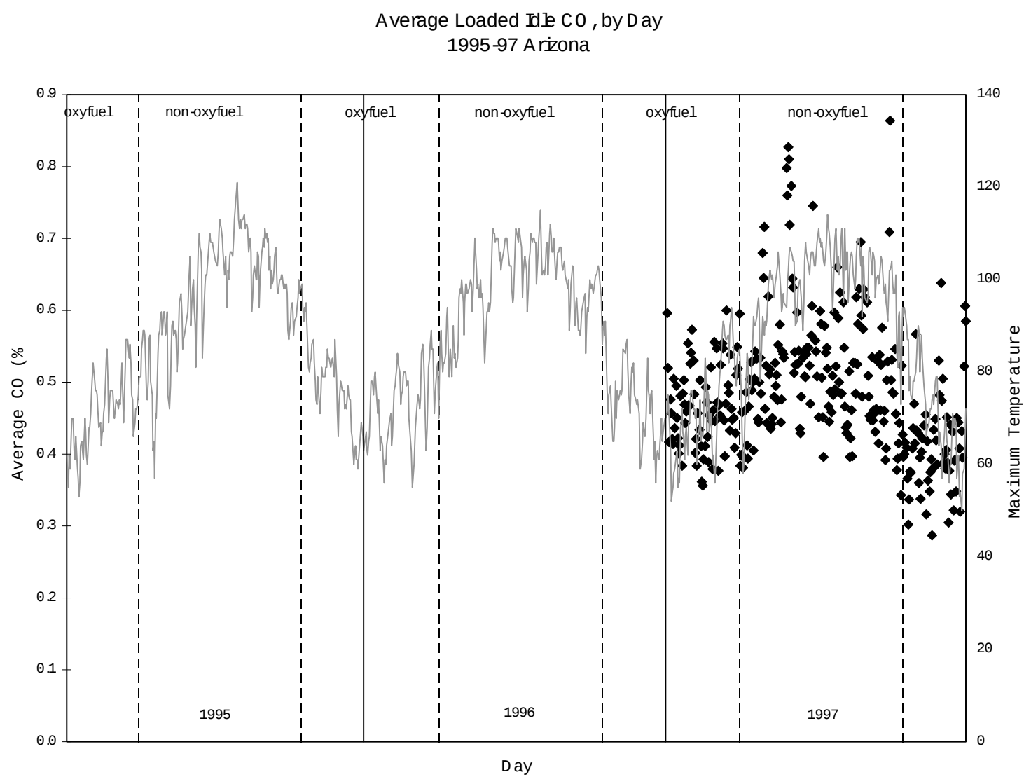
Figure 5.6. Daily Average CO, Arizona Loaded Idle (Pima County)
